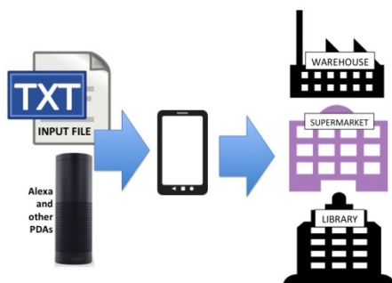
Figure 9. List Integration
